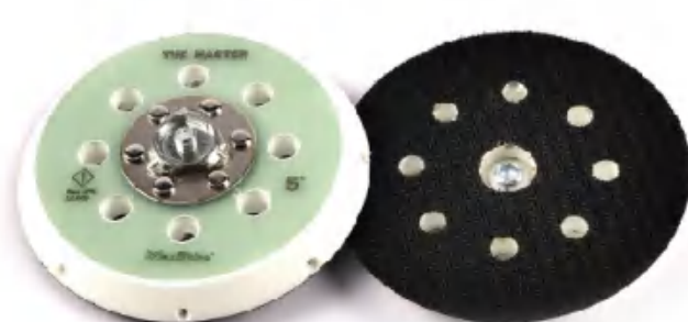
3011125P 5" (125mm) Max OPM: 12000 Thread: 5/16"-24 Hole: 8
